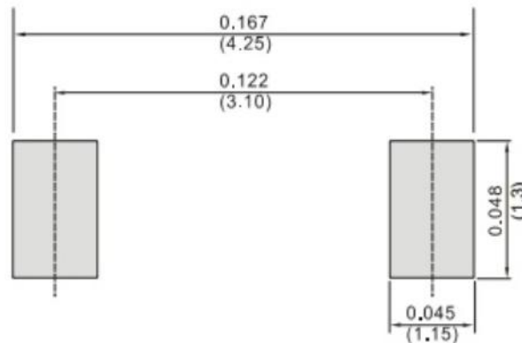
Suggested PCB Solder Layout (mm)
