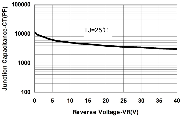
Fig.1-Typical Junction Capacitance
