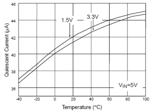
Fig. 6 Quiescent Current vs. Temperature
