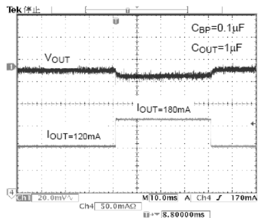
Fig. 12 Load Transient Response
