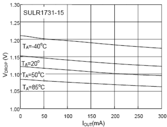
Fig. 9 V DROP VS. I LOAD
