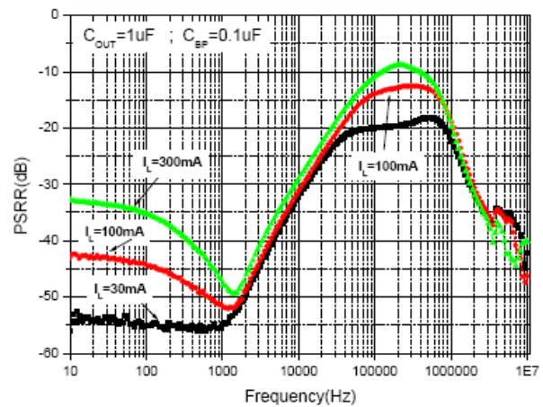
Fig. 18 Ripple Rejection
