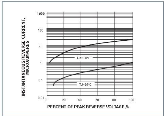
FIG. 4-TYPICAL REVERSE CHARACTERISTICS
